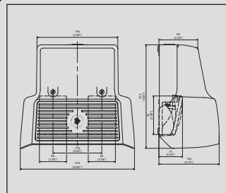
F2 UN – Foot switch with two pedals and protective hood
