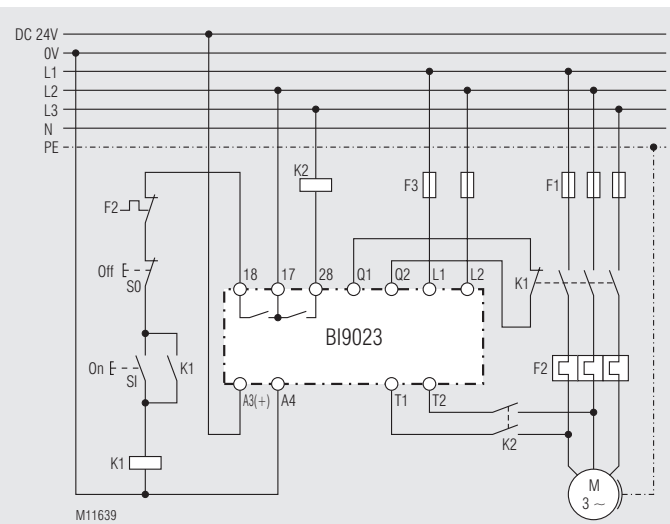
BI 9023 with U_H = DC 24 V
