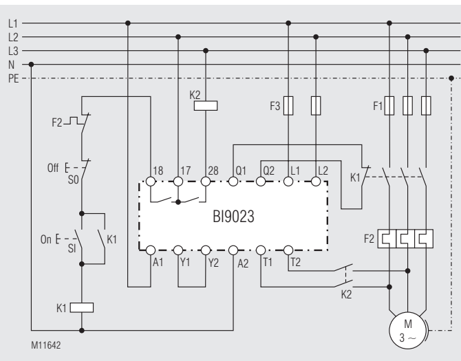
BI 9023 with U_H = AC 230 V
