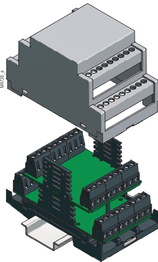
printed circuit board terminal
