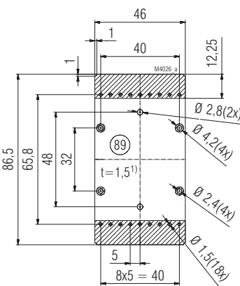
PCB in PCB-position Bottom for 2 x 9-pole contact tag row (plug in screw terminals e.g. plug in cage clamp terminals)
