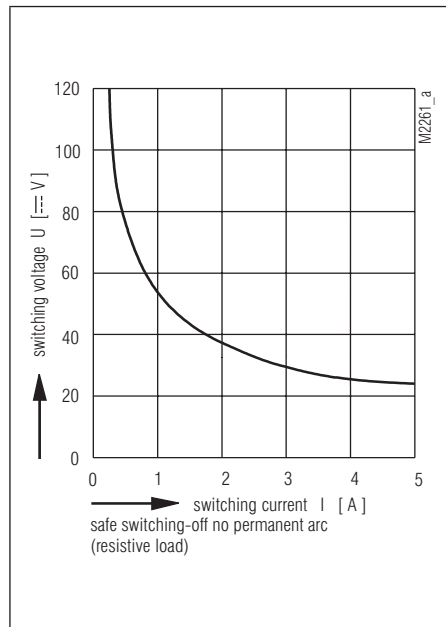
Limit curve for arc-free operation at t_v = 20^\circ\text{C} ) for OW 5691 and OW 5699
