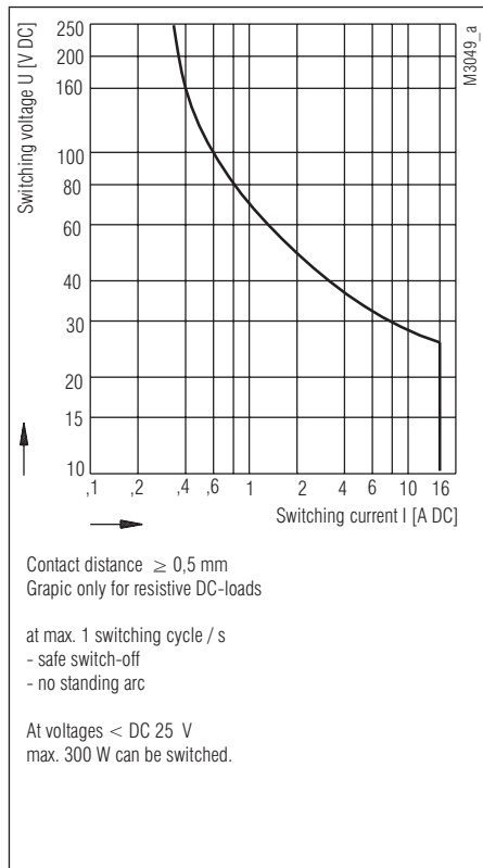
Limit curve for arc-free operation
