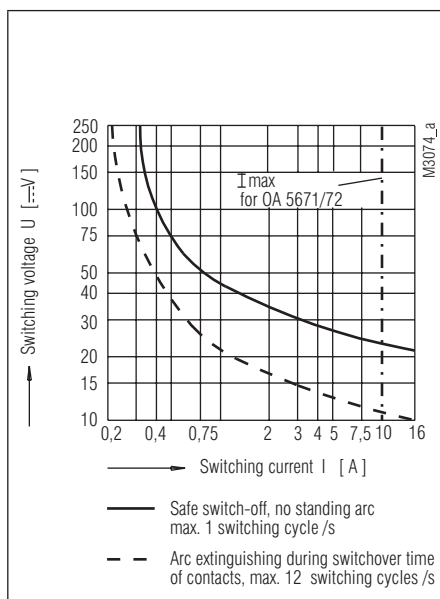
Limit curve for arc-free operation
