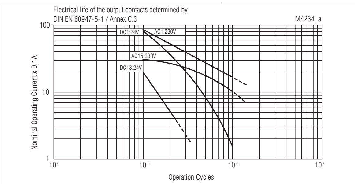
Electrical life for contact material AgNi
