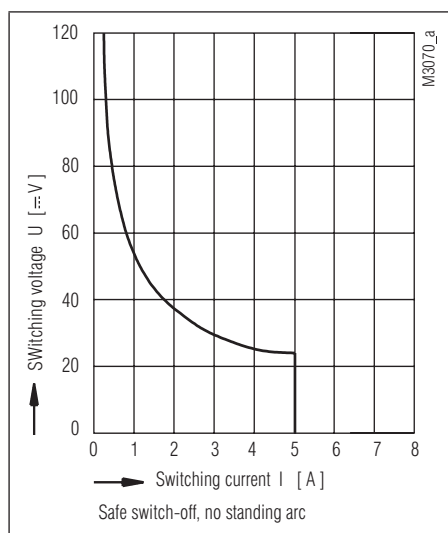
Limit curve for arc-free operation (load limit curve)
