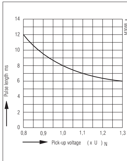
Response-impulse length
