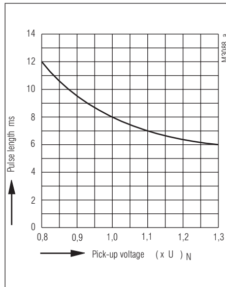
Response-impulse length
