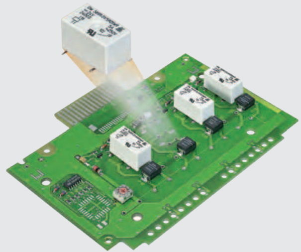
The miniature relays from DOLD are distinguished through their small dimensions with high power and reliability. These mini-relays measure just 10 x 20 x 12 mm. Nonetheless, the switch contacts can easily deal with a continuous current of up to 8 A. In addition, the user can choose between different contact materials and contact designs.
