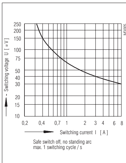
Limit curve for arc-free operation (at t_v = 20^\circ\text{C} )
