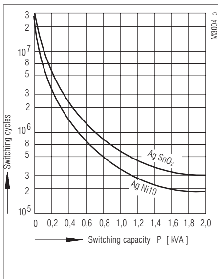
Contact service life (at t_v = 20^\circ\text{C} )
