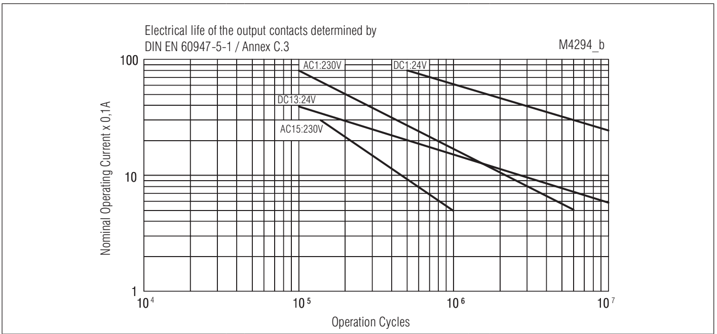
Electrical life
