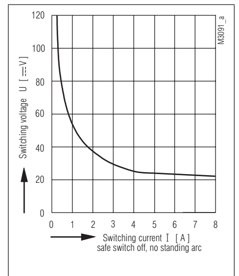
Limit curve for arc-free operation
