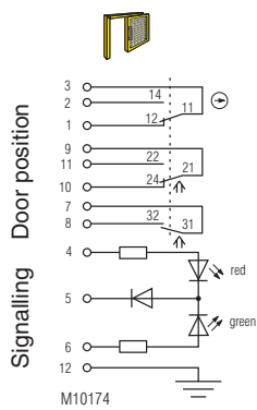
Fig. 2: Lock deactivated: 2nd key removed, Actuator removed, 1st key inserted Door open
