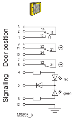
Fig. 1: Locked while activated: Actuator inserted, 2nd key inserted, 1st key removed Door closed
