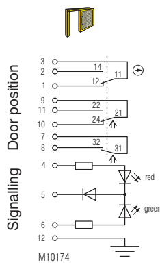
Fig. 2: Locking module deactivated: Key (top) inserted, Actuator (bottom) removed Door unlocked and open
