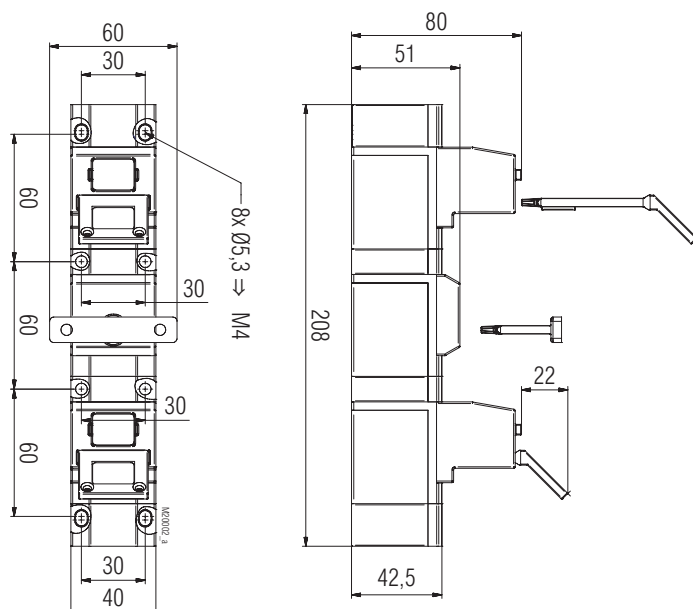
M10B01M/K Clearance tolerances \pm 2\%
