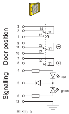
Fig. 1: Locked while activated: Actuator inserted, 2nd key inserted, Actuator removed, 1st key removed Door closed
