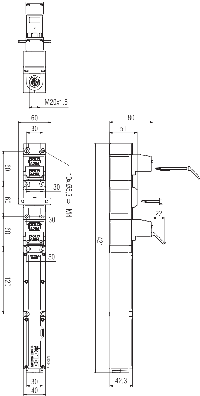
YRX10B01M/K Clearance tolerances ± 2%
