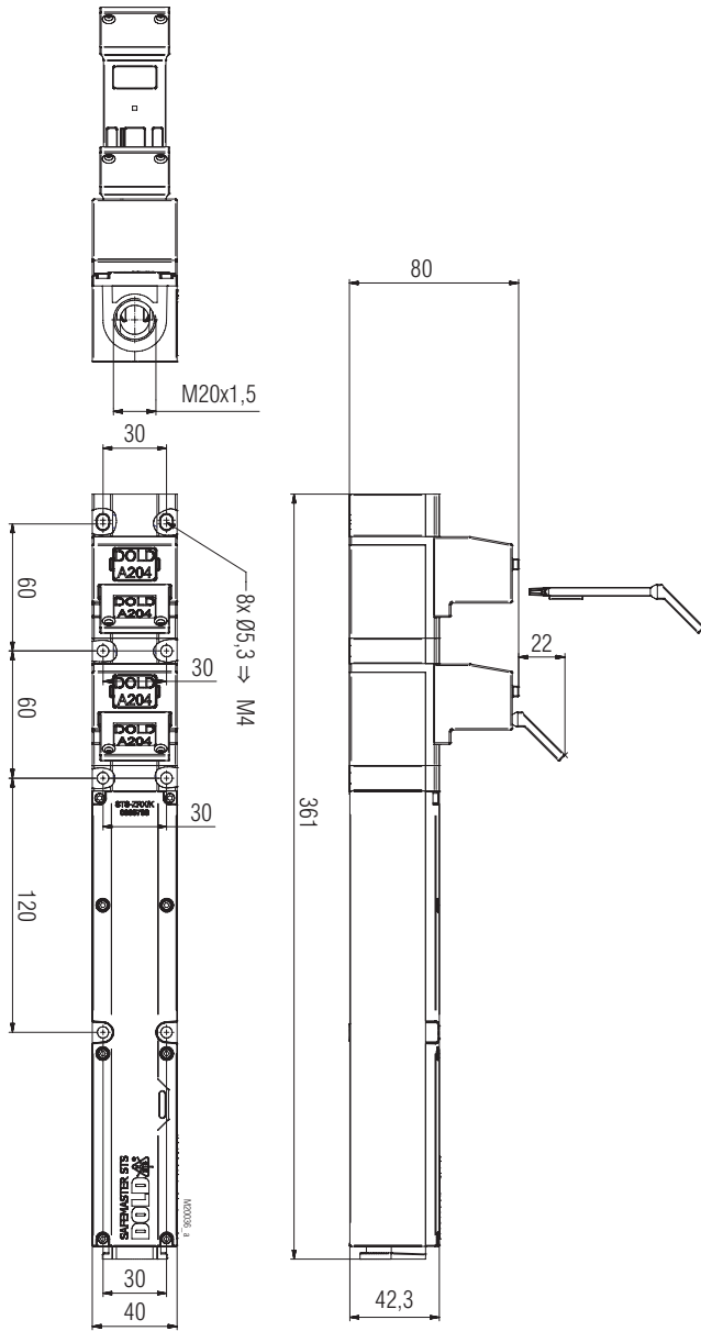
YRX11M/K Clearance tolerances \pm 2\%
