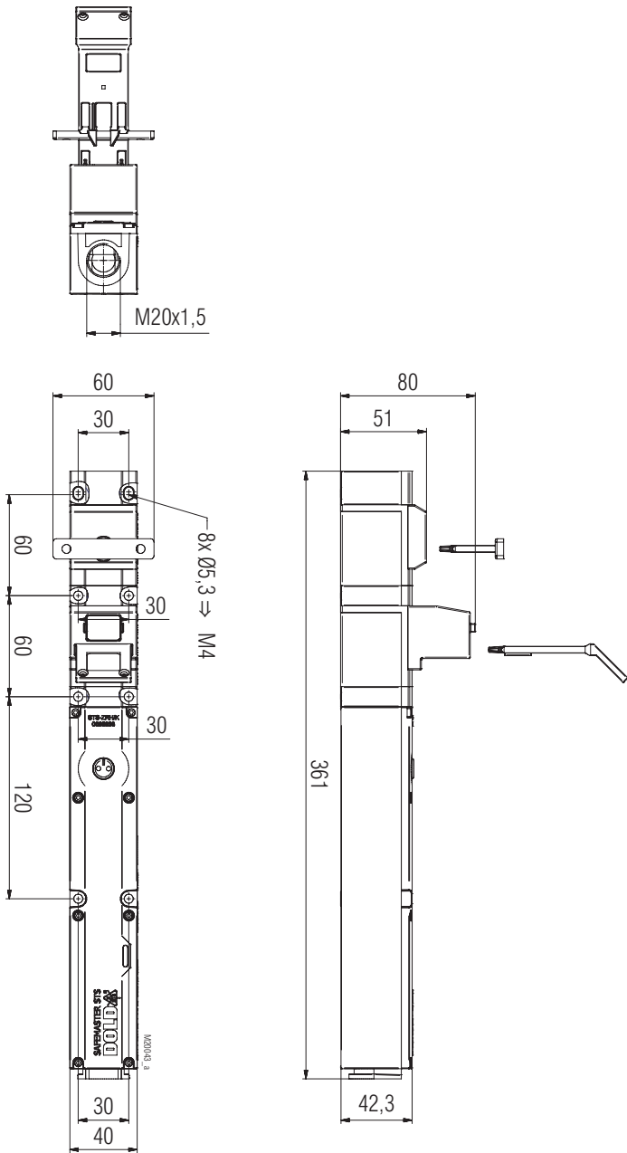
ZRH01BM/K Clearance tolerances \pm 2\%
