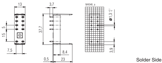
Solder Side
