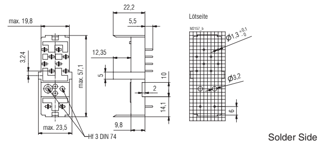
Solder Side
