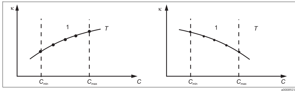
Fig. 36: Measured data for a constant process temperature (example)
