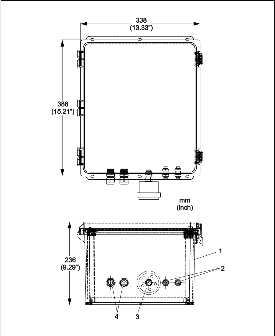
Fig. 5: Enclosure Detail
