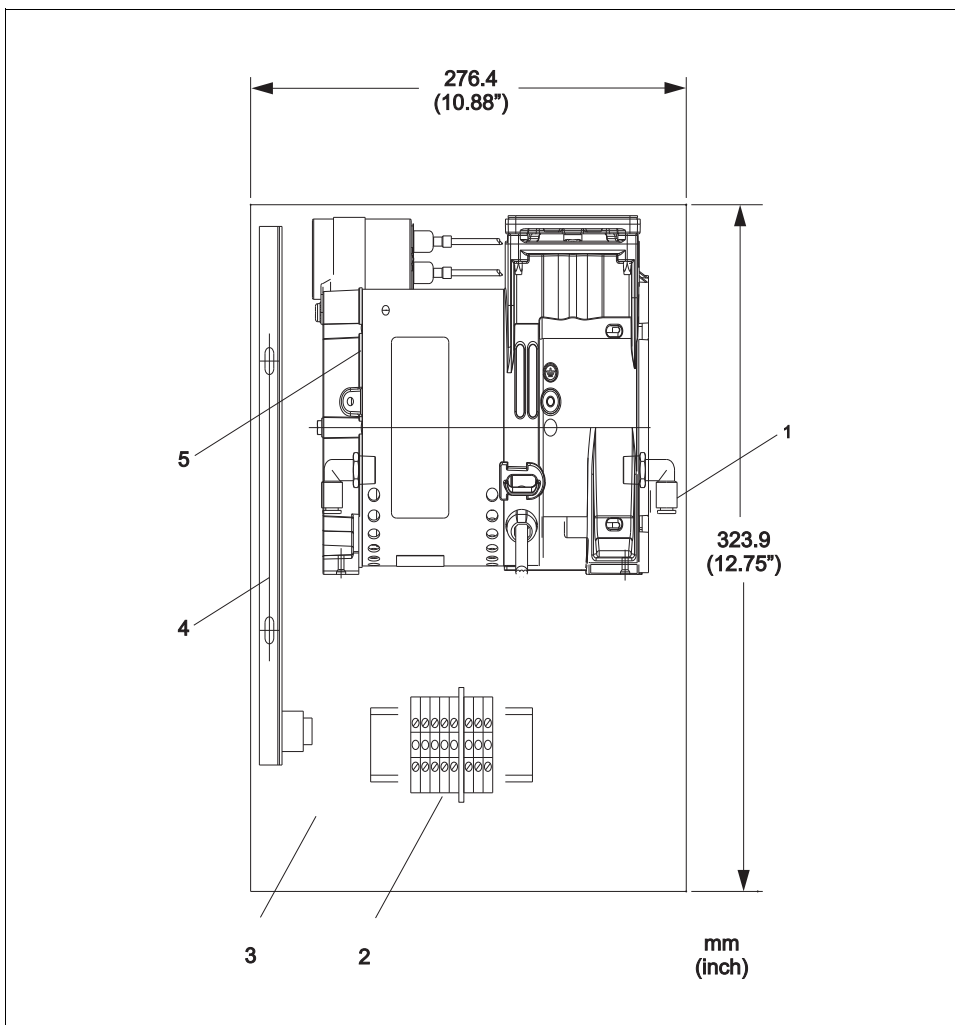
Fig. 1: Sensor installation - Front view
