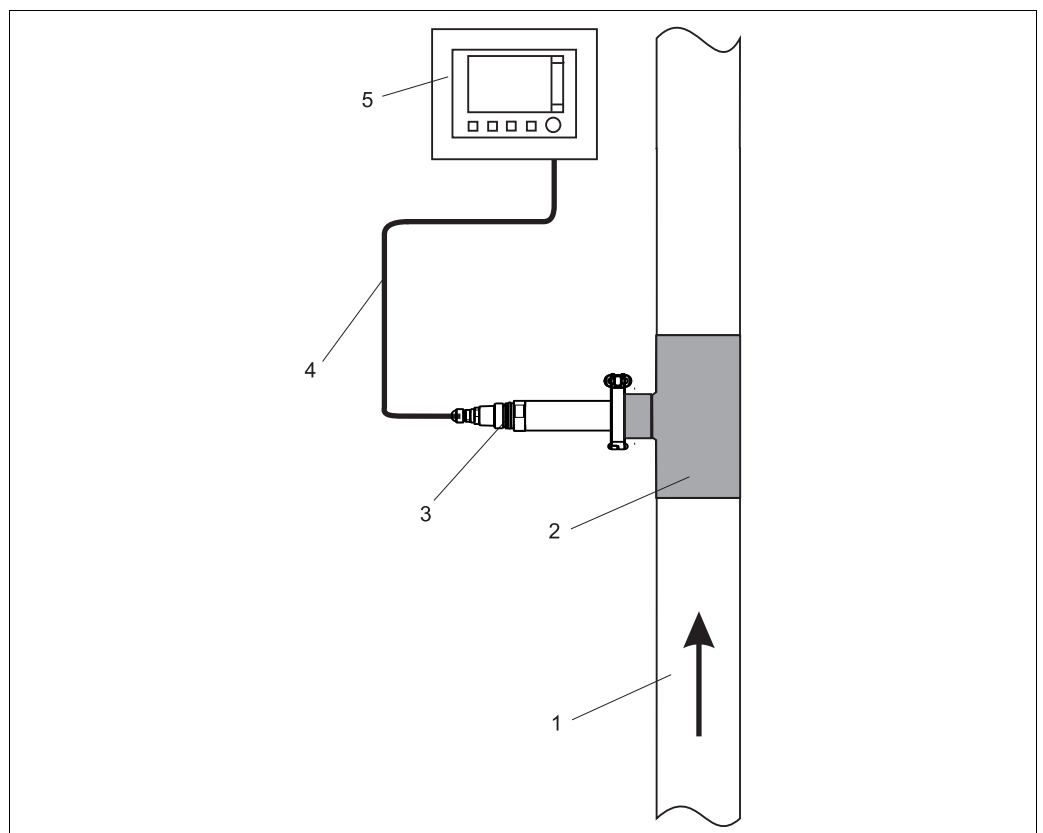
Fig. 2: Installation in the process pipe
