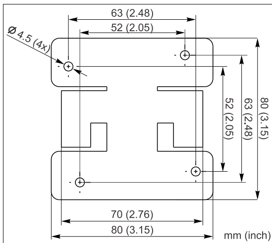
Dimensions of the mounting plate
