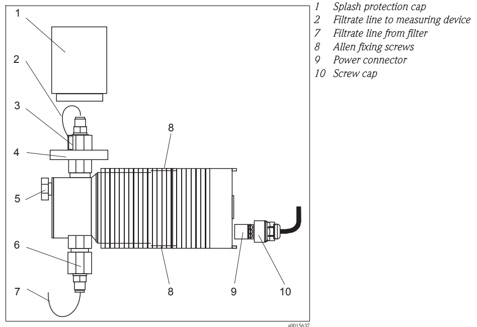
Fig. 30: Membrane pump
