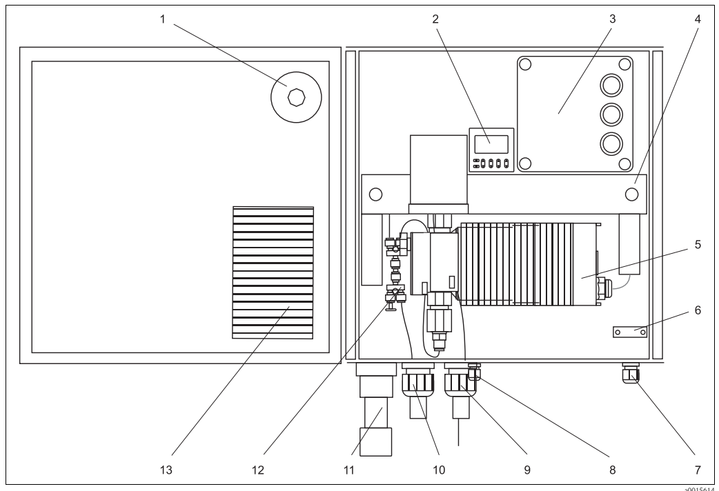
Fig. 10: Control box
