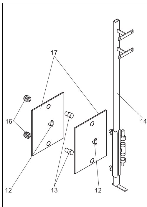
Fig. 36: Filter element holder for basin
