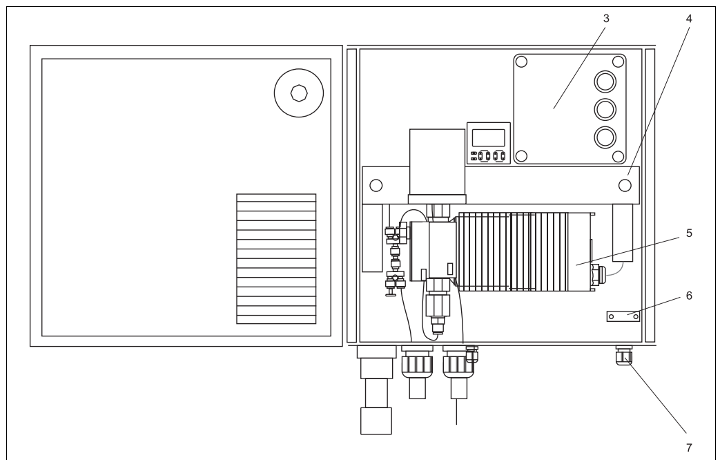
Fig. 14: Control box
