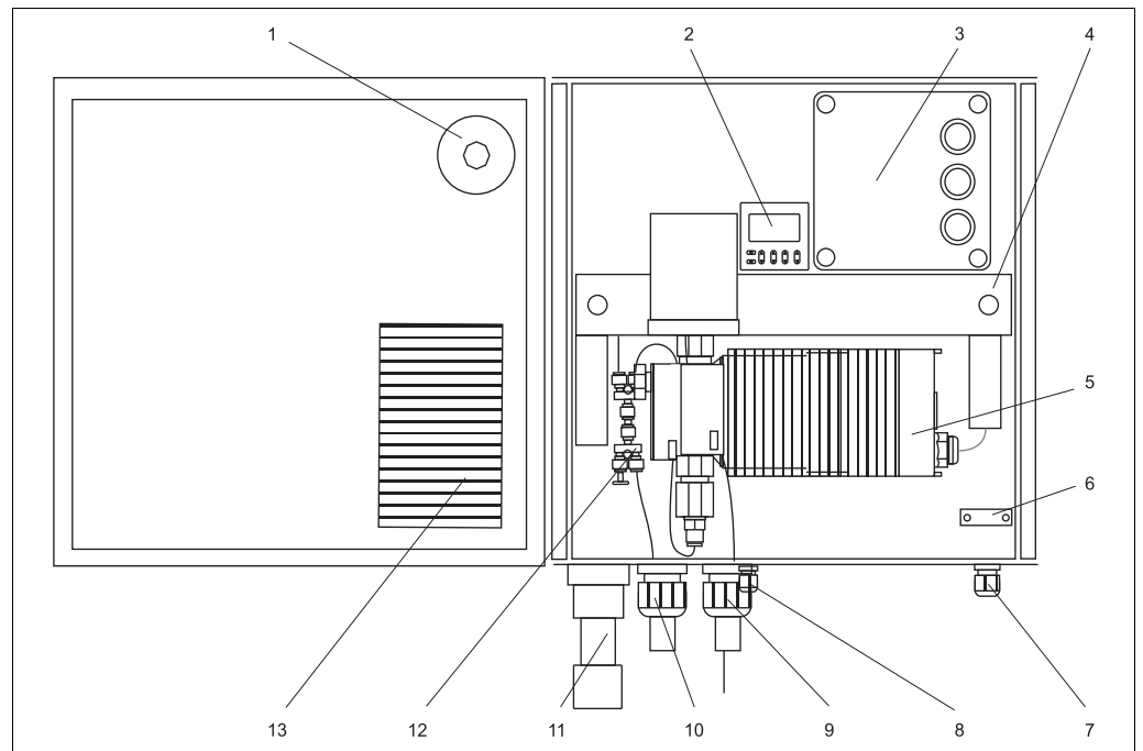
Fig. 20: Control box
