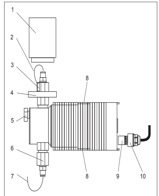
Fig. 12: Membrane pump
