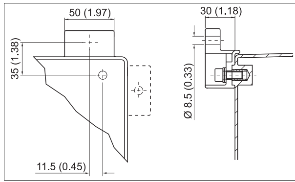
Fig. 8: Wall brackets
