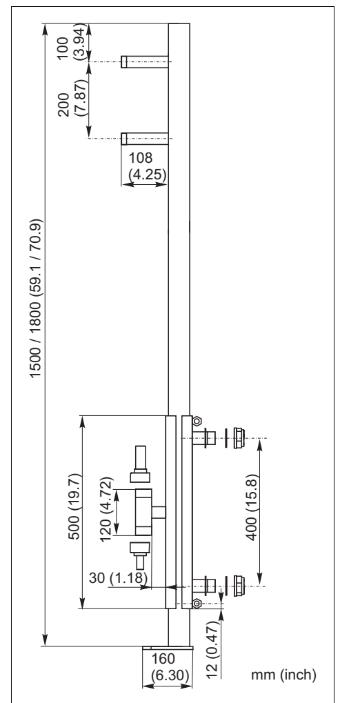
Fig. 32: Holder for basin, side view
