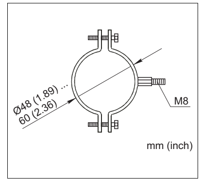
Fig. 9: Pipe clamp for rail mounting
