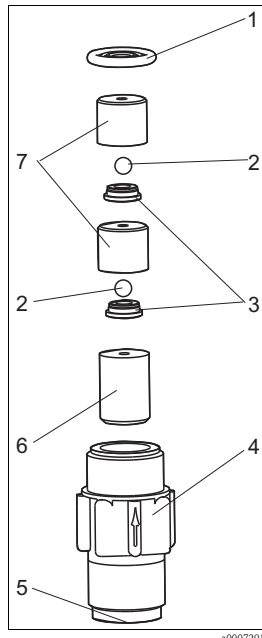
Fig. 28: Suction valve
