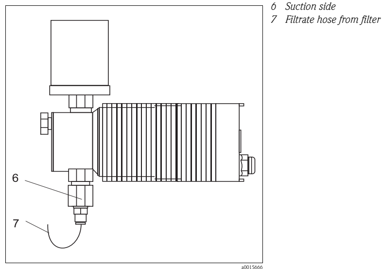
Fig. 25: Membrane pump
