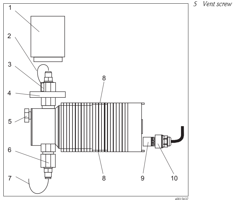
Fig. 22: Membrane pump
