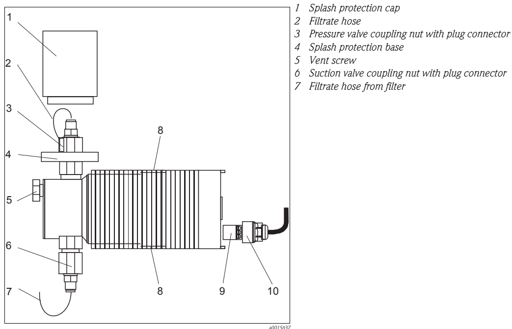
Fig. 26: Membrane pump
