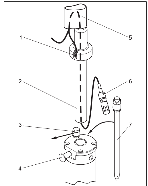
Fig. 22: Sensor installation
