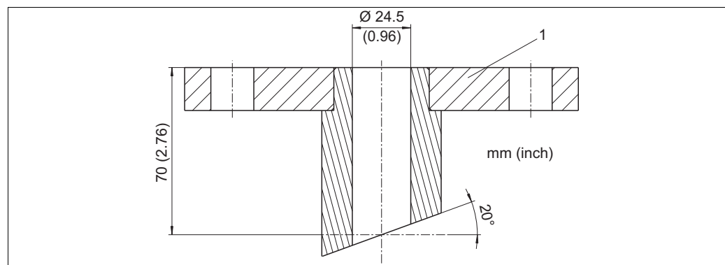
Fig. 41: Welded fitting
