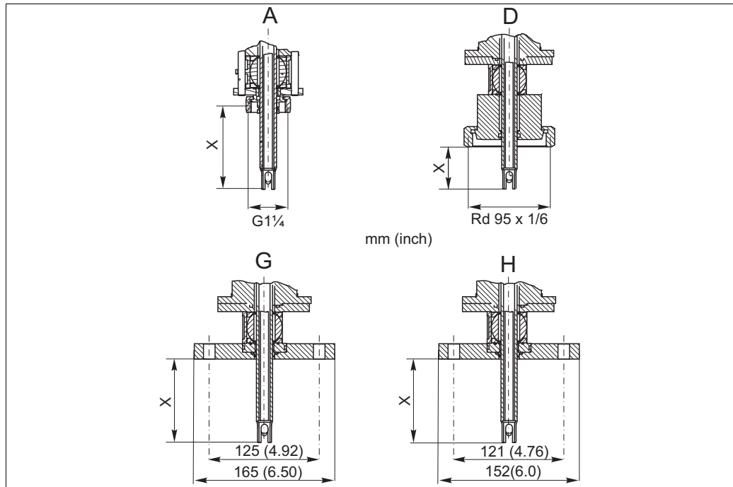
Fig. 5: Process connections
