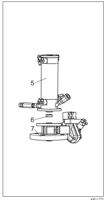
Fig. 35: Dismantling part 3
