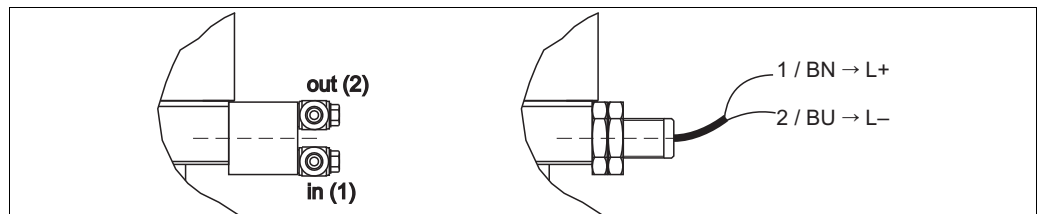
Fig. 10: Limit position switches, left: pneumatic (1 = compressed air inlet, 2 = compressed air outlet) right: electric (NAMUR)
