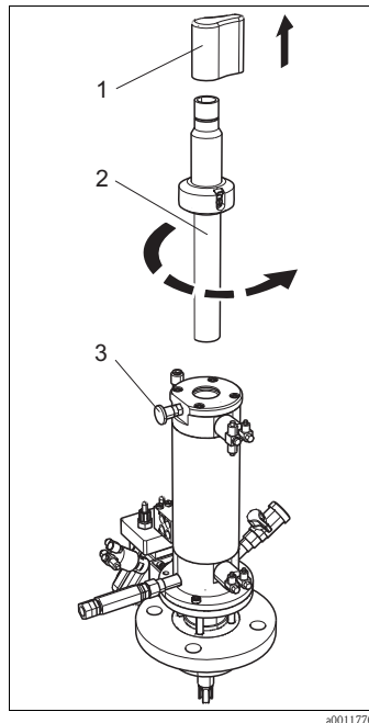
Fig. 33: Dismantling part 1
