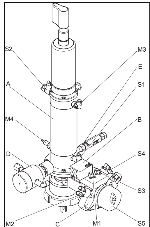
Fig. 27: Electrical limit position switches
