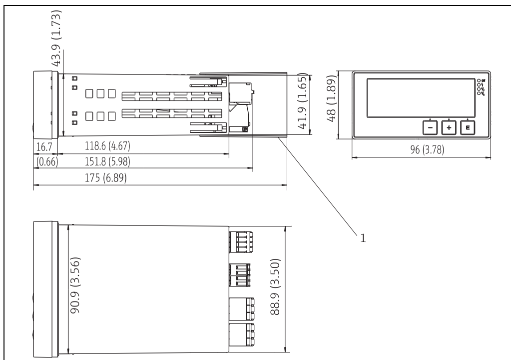
Dimensions of the panel meter in mm (in)
