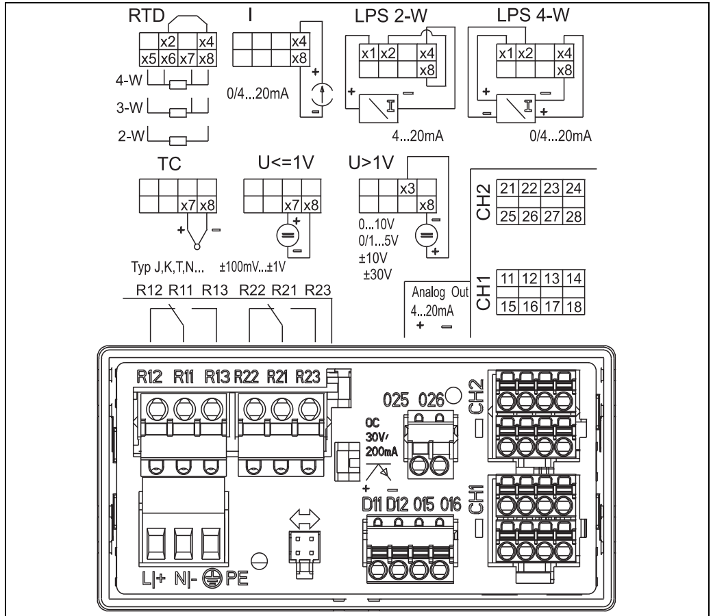
Terminal assignment of panel meter (relays (terminals Rx1-Rx3) and channel 2 (terminals 21-28 and O25/O26) are optional)
