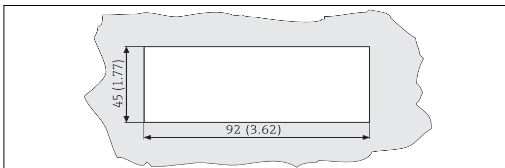
Panel cutout, dimensions in mm (in)
