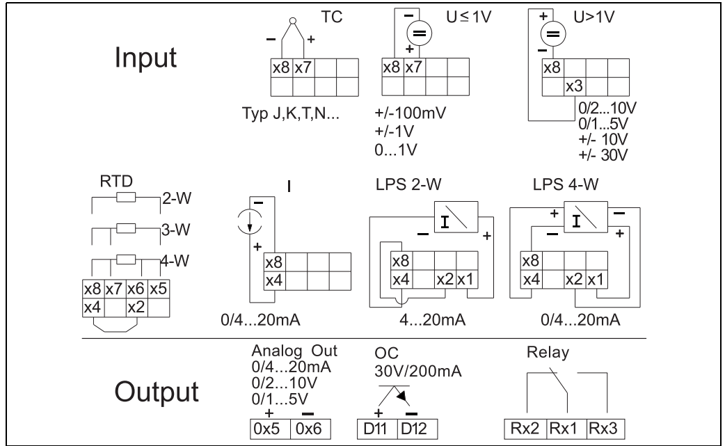
Terminal assignment of the process transmitter (relays (terminals Rx1-Rx3) and channel 2 (terminals 21-28 and O25/O26) are optional)
