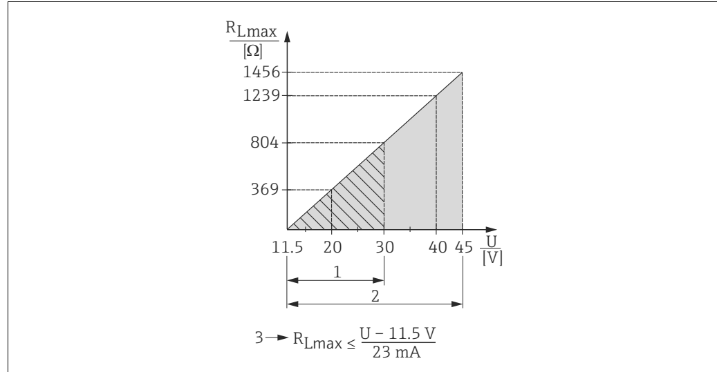
Load diagram
