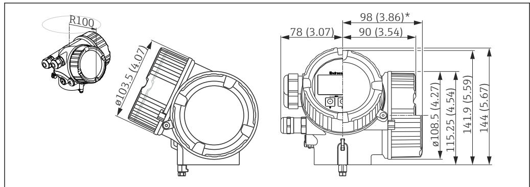
22 Housing GT18 (316L); Dimensions in mm (in) *for devices with integrated overvoltage protection.
