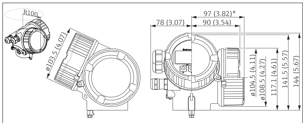
24 Housing GT20 (Alu coated); Dimensions in mm (in) *for devices with integrated overvoltage protection.
