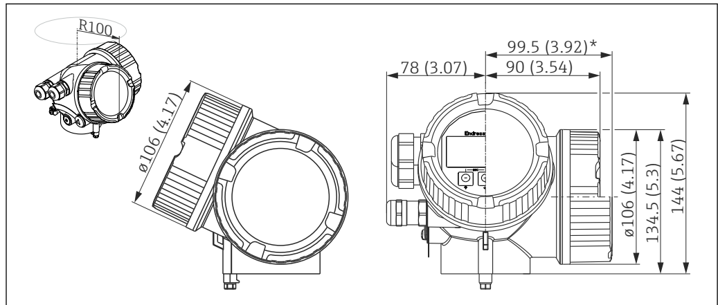
23 Housing GT19 (Plastics PBT); Dimensions in mm (in) *for devices with integrated overvoltage protection.
