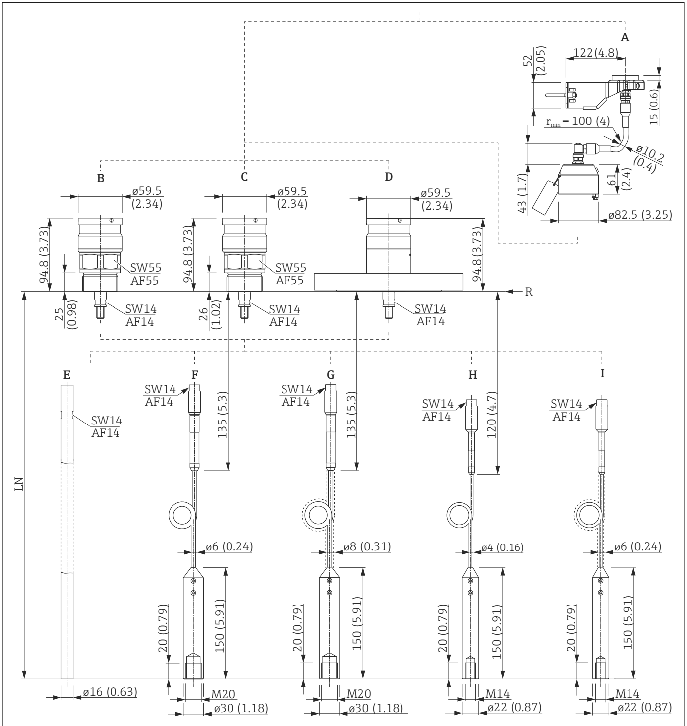
27 FMP57: Process connection / probe. Unit of measurement mm (in)
