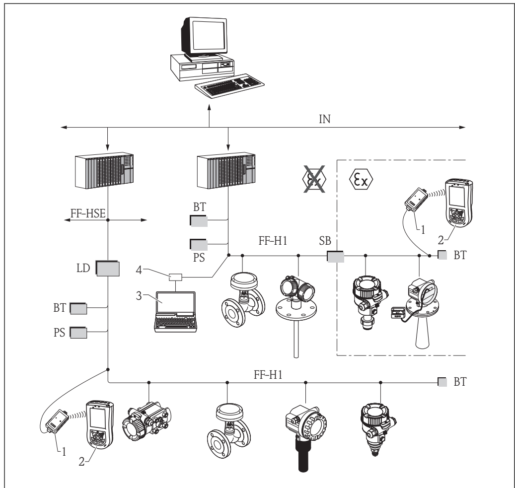
30 FOUNDATION Fieldbus system architecture with associated components
