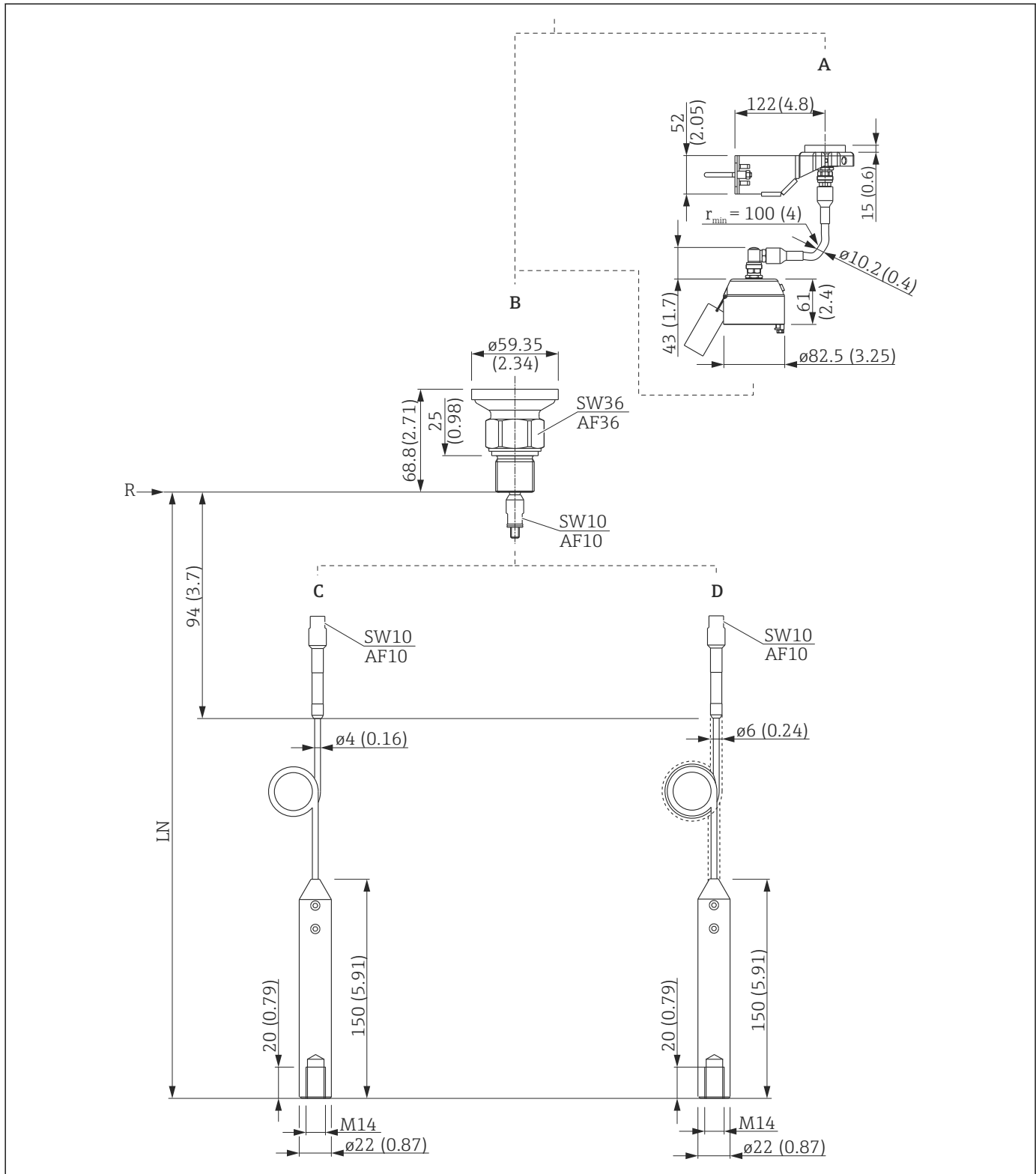
26 FMP56: Process connection / probe. Unit of measurement mm (in)
