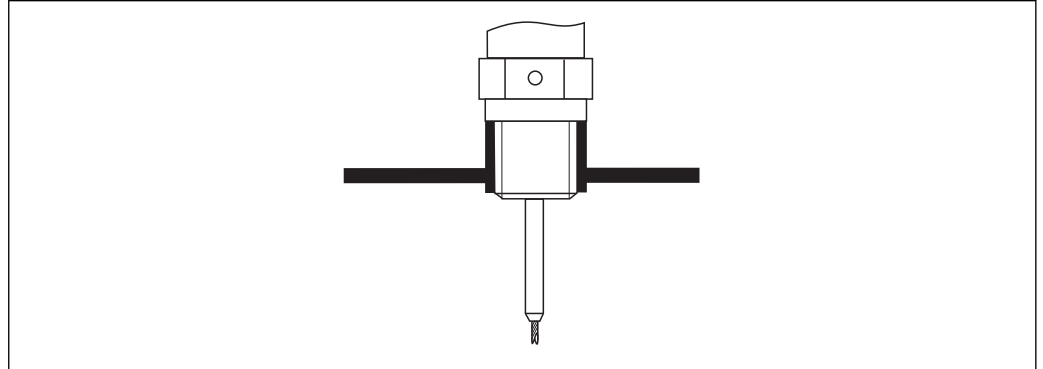
19 Mounting with threaded connection; flush with the container ceiling
