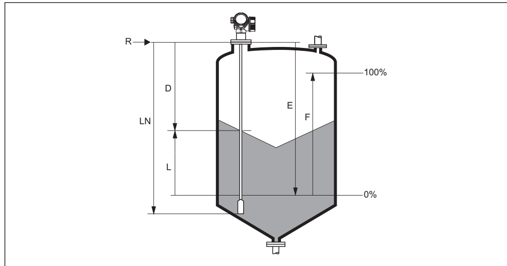
1 Parameters for level measurement with the guided radar
