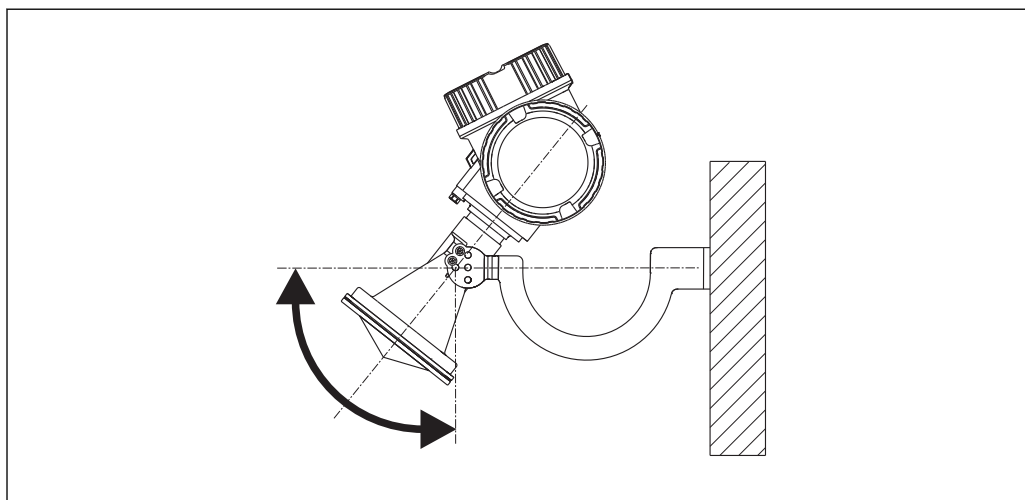
13 Installation of the horn antenna with mounting bracket
