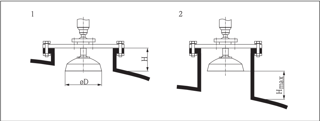
15 Nozzle mounting of Micropilot FMR57 with parabolic antenna
