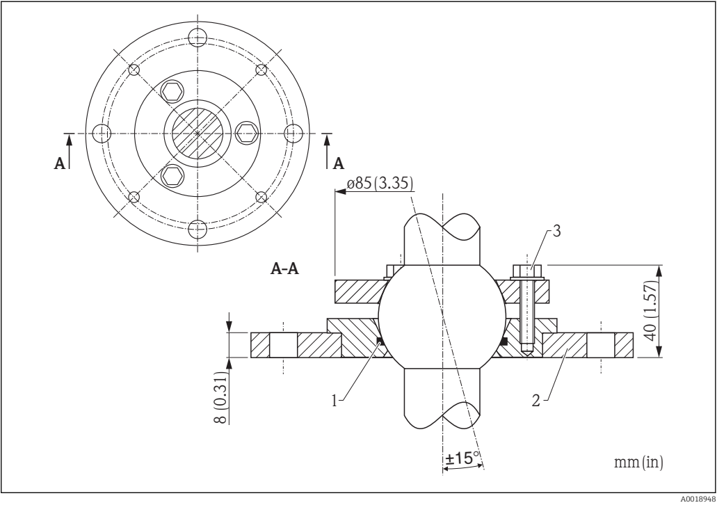
Alignemnt device with Endress+Hauser UNI flange
