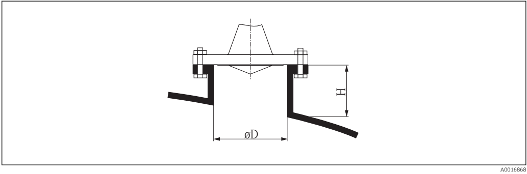
12 Nozzle height and diameter for horn antenna with slip-on flange
