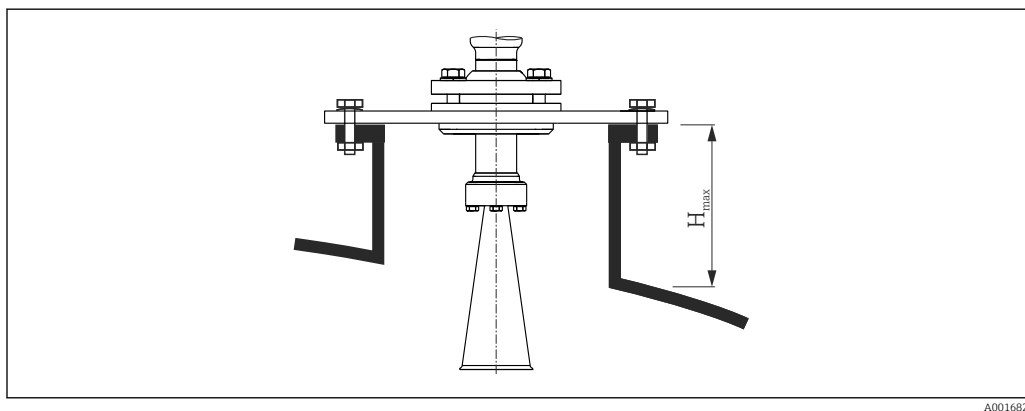
14 Nozzle height for the horn antenna (FMR57)
