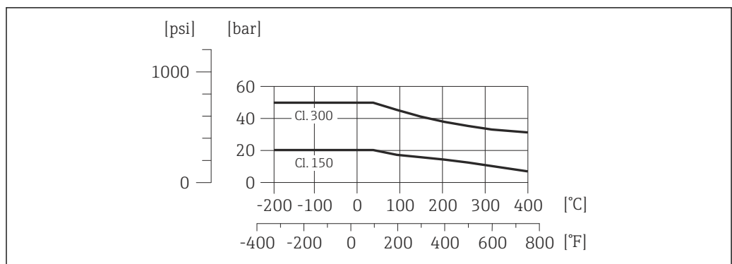
19 Process connection material: stainless steel, multiple certifications, 1.4404 (F316, F316L)
