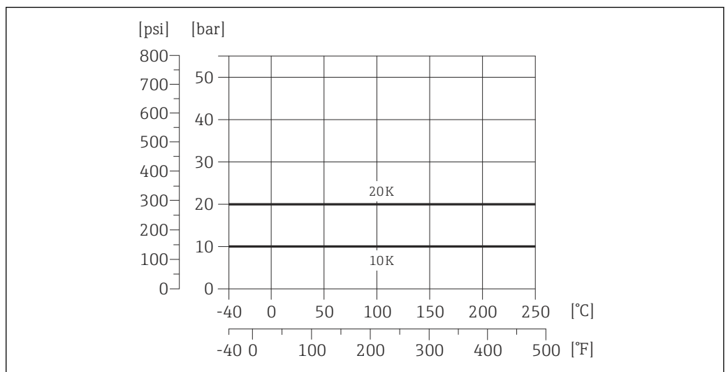
22 Process connection material: cast alloy CX2MW similar to Alloy C22/2.4602
