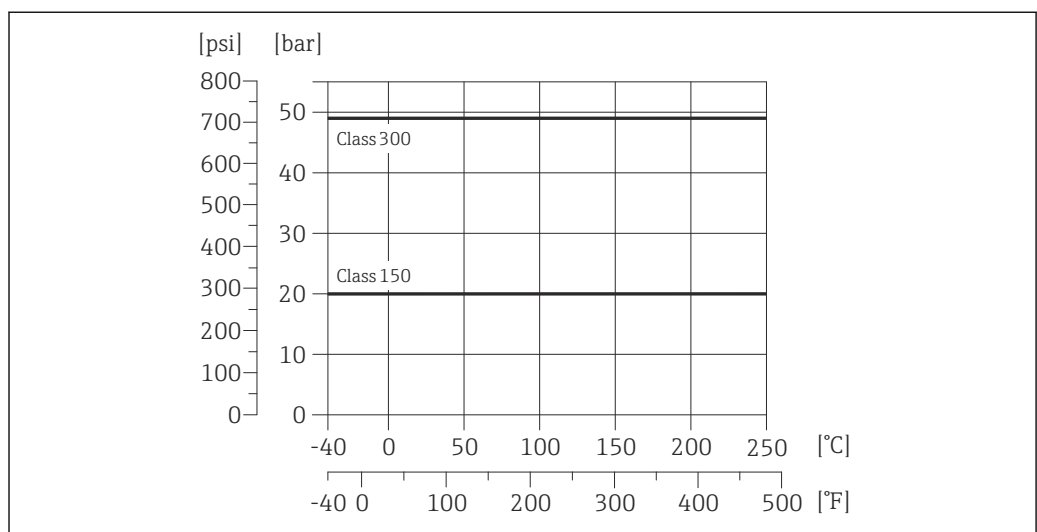
20 Process connection material: cast alloy CX2MW similar to Alloy C22/2.4602
