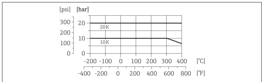
19 Process connection material: stainless steel, multiple certifications, 1.4404 (F316, F316L)
