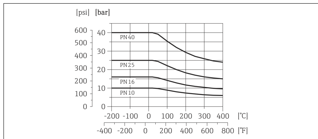
17 Process connection material: stainless steel, multiple certifications, 1.4404 (F316, F316L)
