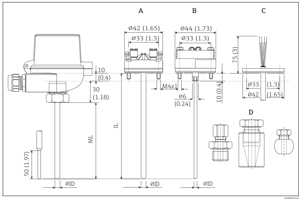
4 Dimensions of the Omnigrad T TR24
