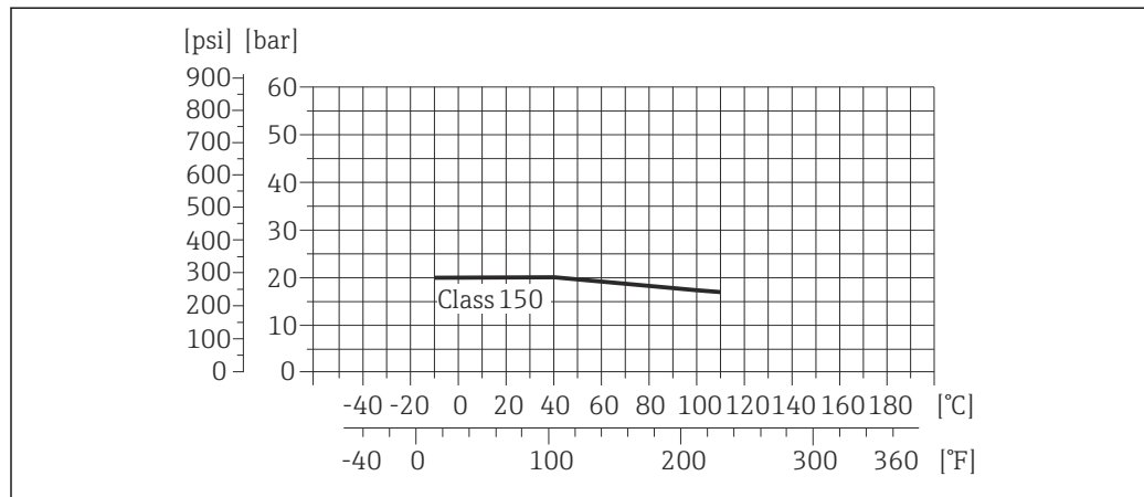
17 Process connection material: carbon steel, A105
