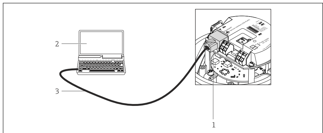
23 Connection for order code for "Output", option L: PROFIBUS DP
