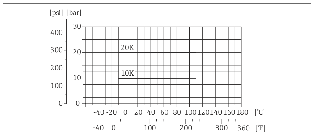
18 Process connection material: carbon steel, S235JRG2/HII
