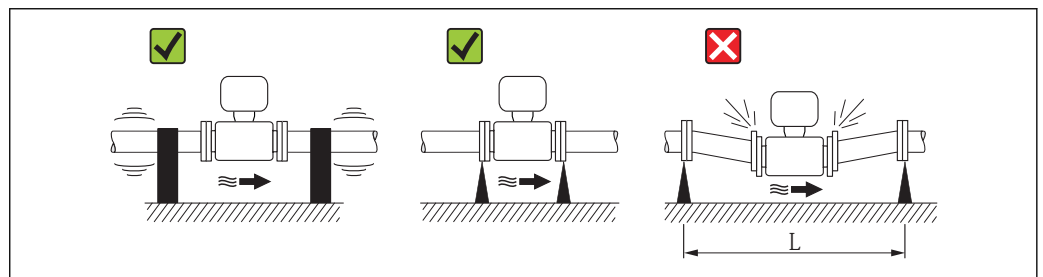
19 Measures to avoid device vibrations (L > 10 m (33 ft))
