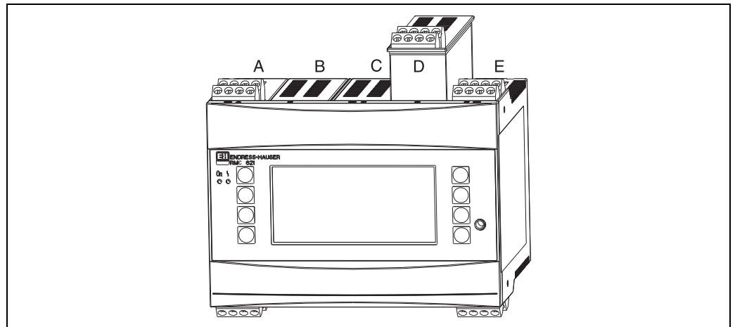
RMC621 upgrade with expansion cards (optional or available as accessories)
