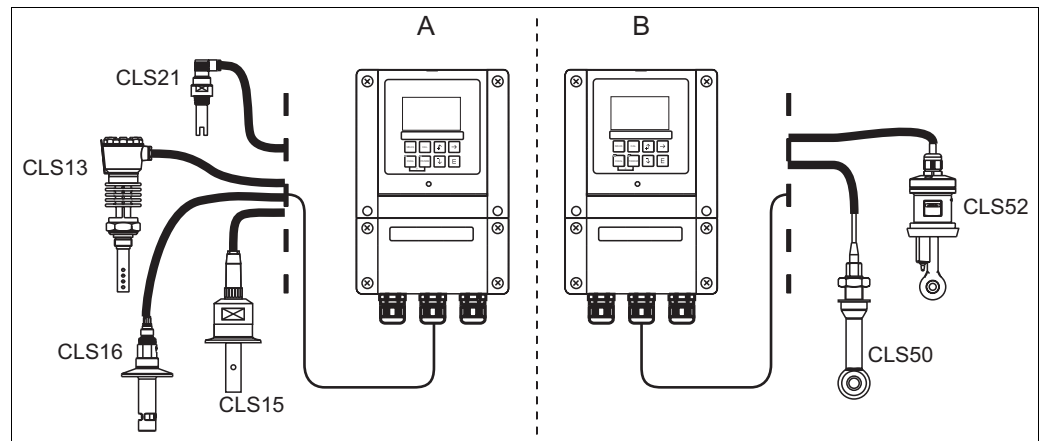
Measuring system
