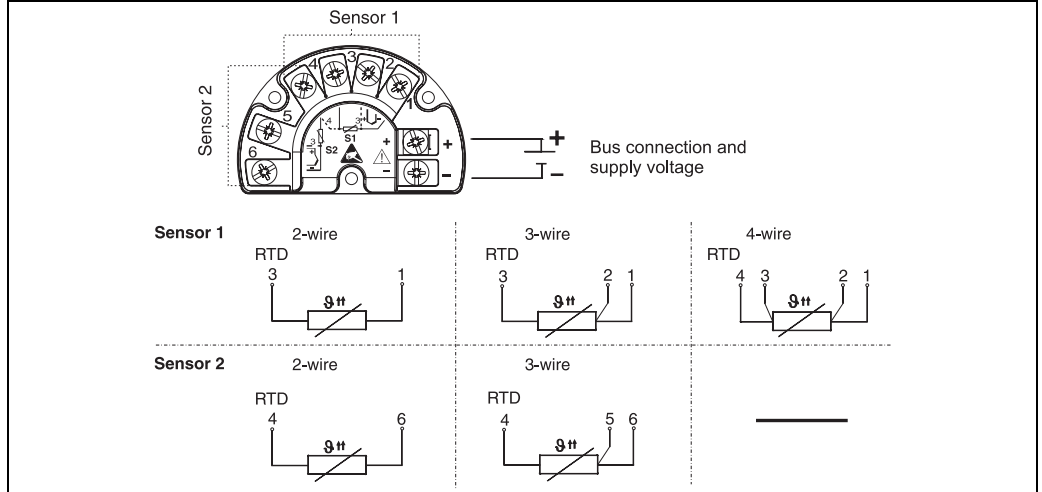
Electrical connection
