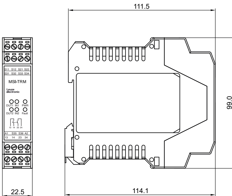
Figure 14.1: Dimensions MSI-TRMB-01
