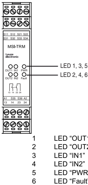
Figure 3.3: Display elements of the MSI-TRM
