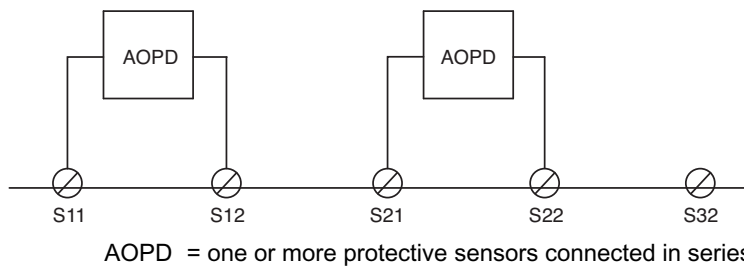
Figure 4.2: Basic wiring for operating mode 2 AOPDs (two protective sensors)
