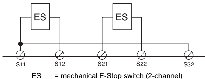
Figure 4.3: Basic wiring of operating mode ES (E-Stop)
