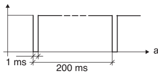
a Test signal of MSI-TRM at S11 and S21
