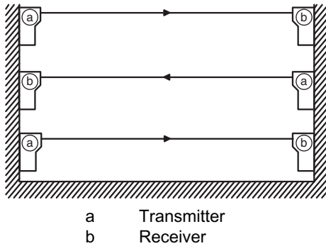
Figure 6.1: Multi-axis arrangement
