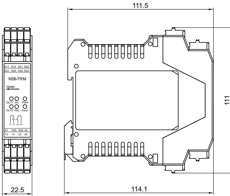
Figure 14.2: Dimensions MSI-TRMB-02
