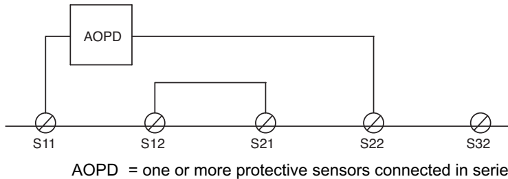
Figure 4.1: Basic wiring for operating mode 1 AOPD (one protective sensor)
