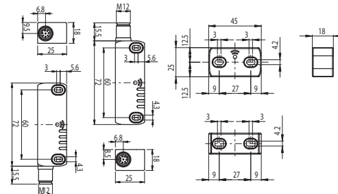
Figure 6: Dimensional drawing
