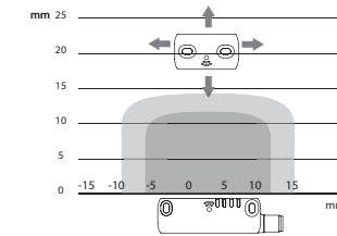
Figure 4: Approach directions
