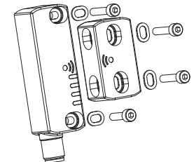
Figure 5: Mounting
