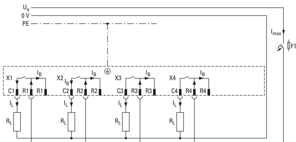
Figure 48: Wiring diagram with U_e at all four connection terminals for total currents > 10\text{ A}
