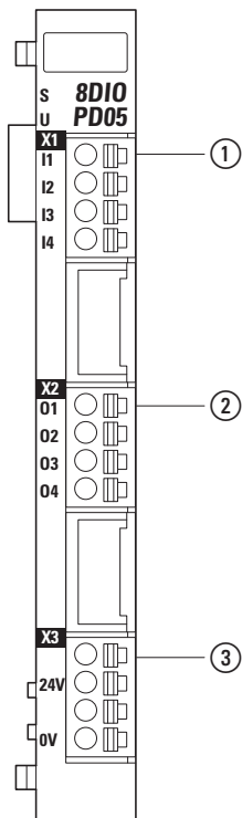
Figure 63: Pin assignment
