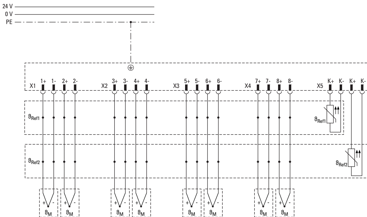
Figure 92: Wiring example with 8 thermocouples and 2 KTY sensors; the \theta_M measuring points and the \theta_{Ref1} and \theta_{Ref2} reference junctions are clearly shown
