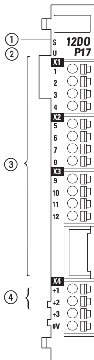
Figure 54: LED signals and pin assignment
