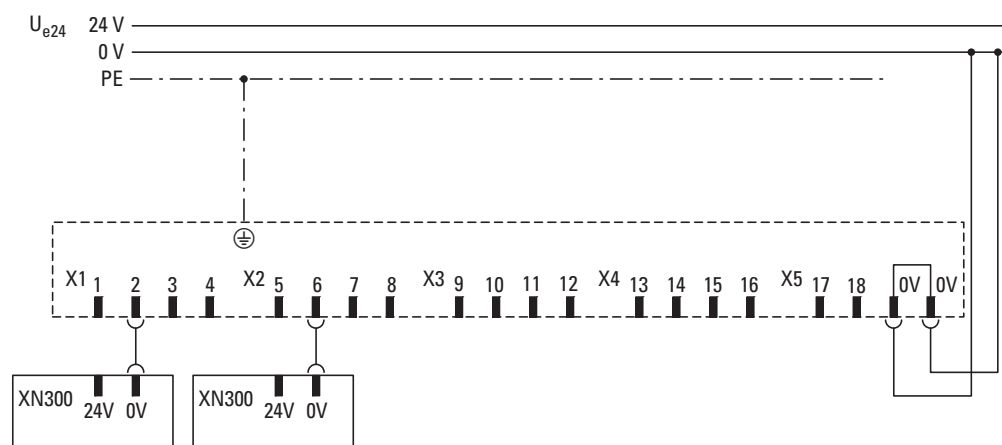
Figure 18: Wiring example
