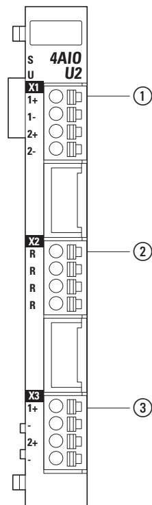
Figure 99: Pin assignment
