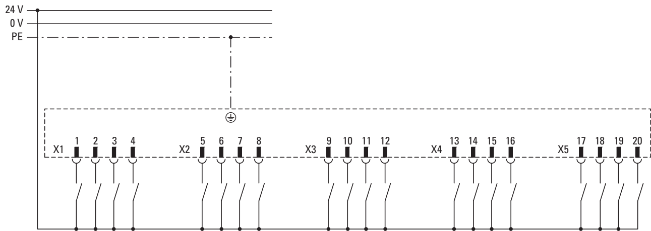
Figure 34: Input wiring
