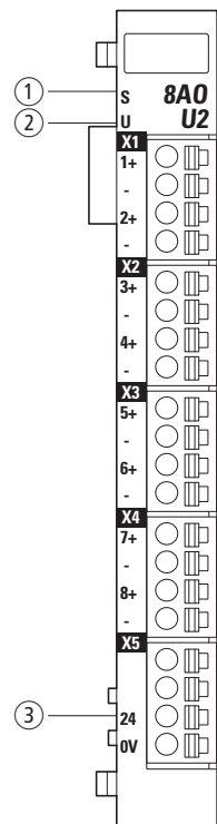
Figure 94: LED signals and pin assignment
