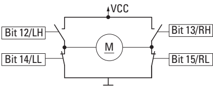
Figure 128: Block diagram showing a motor armature short-circuit
