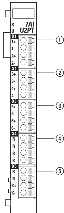
Figure 83: Pin assignment
