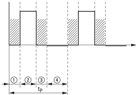
Figure 133: Output signal with clockwise operation ① Motor Off ② Clockwise motor operating direction ③ Motor Off ④ Motor armature short-circuit
