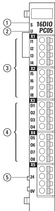
Figure 71: XN-322-16DIO-PC05 LEDs
