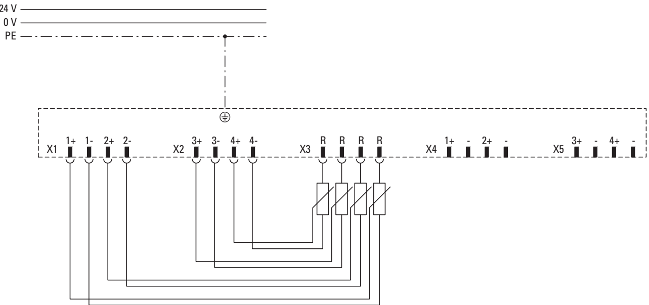
Figure 107: Potentiometer measurement wiring
