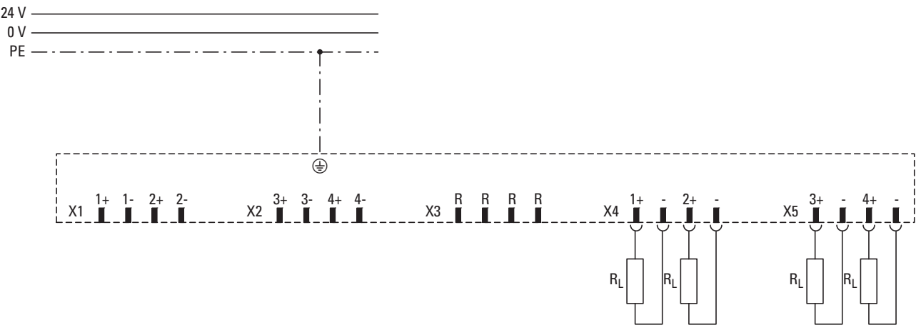
Figure 106: Analog outputs connection
