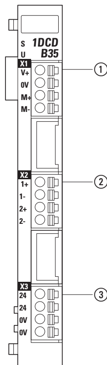
Figure 123: Pin assignment XN-322-1DCD-B35
