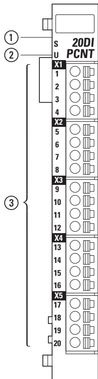
Figure 36: LED signals and pin assignment
