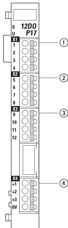
Figure 55: Pin assignment
