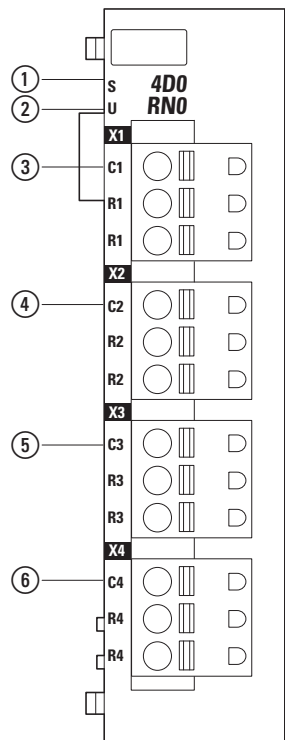
Figure 44: LED signals and pin assignment
