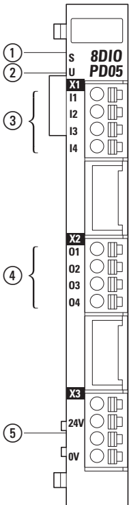
Figure 62: XN-322-8DIO-PD05 LEDs
