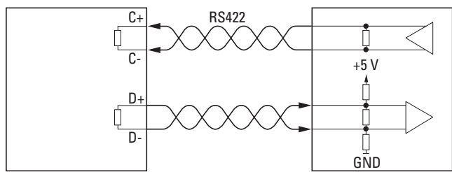
Figure 147: Application Style
