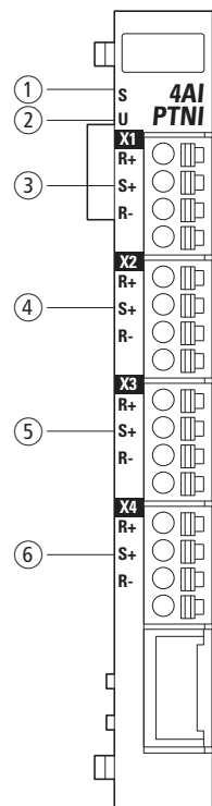
Figure 77: LED signals and pin assignment
