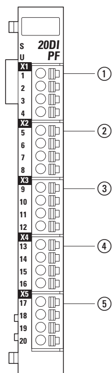
Figure 33: Pin assignment
