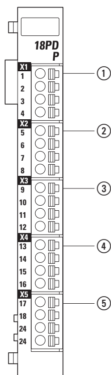
Figure 20: LED signals and pin assignment for XN-322-18PD-P
