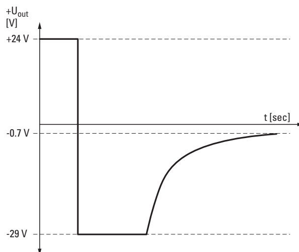
Figure 52: Voltage limiting when switching off inductive loads
