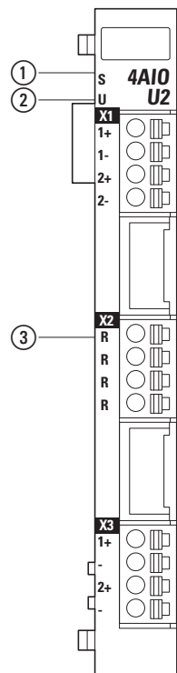
Figure 98: LED signals and pin assignment
