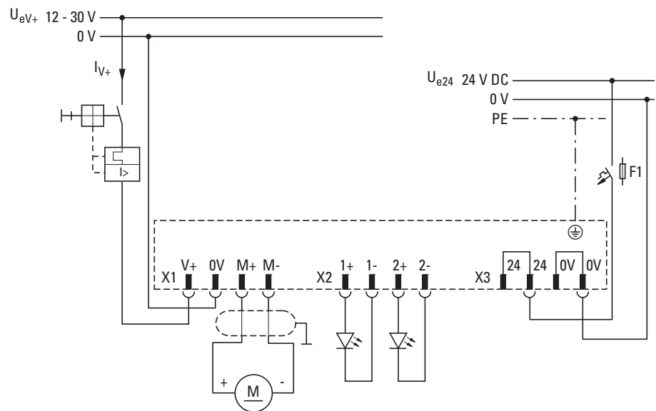
Figure 124: Diagram version 2: Wiring example for XN-322-1DCD-B35
