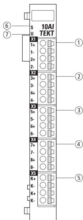
Figure 91: LED signals and pin assignment
