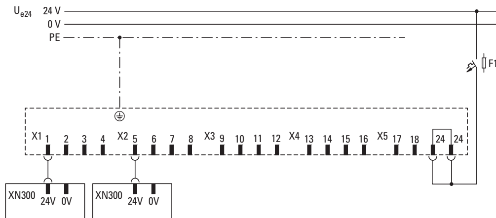
Figure 21: Wiring example
