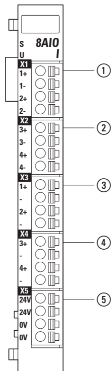
Figure 115: Pin assignment
