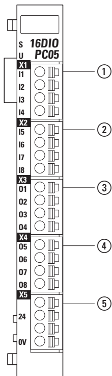
Figure 72: Pin assignment
