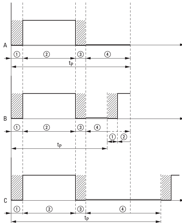
Figure 132: Output signal
