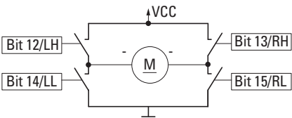
Figure 129: Block diagram showing open motor
