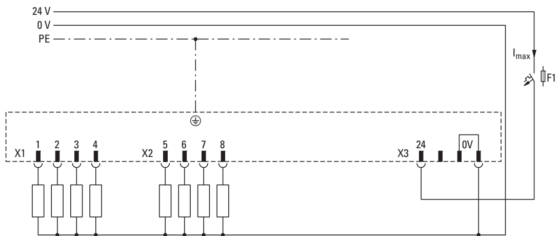
Figure 51: Wiring example
