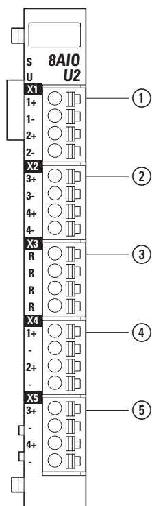
Figure 105: Pin assignment
