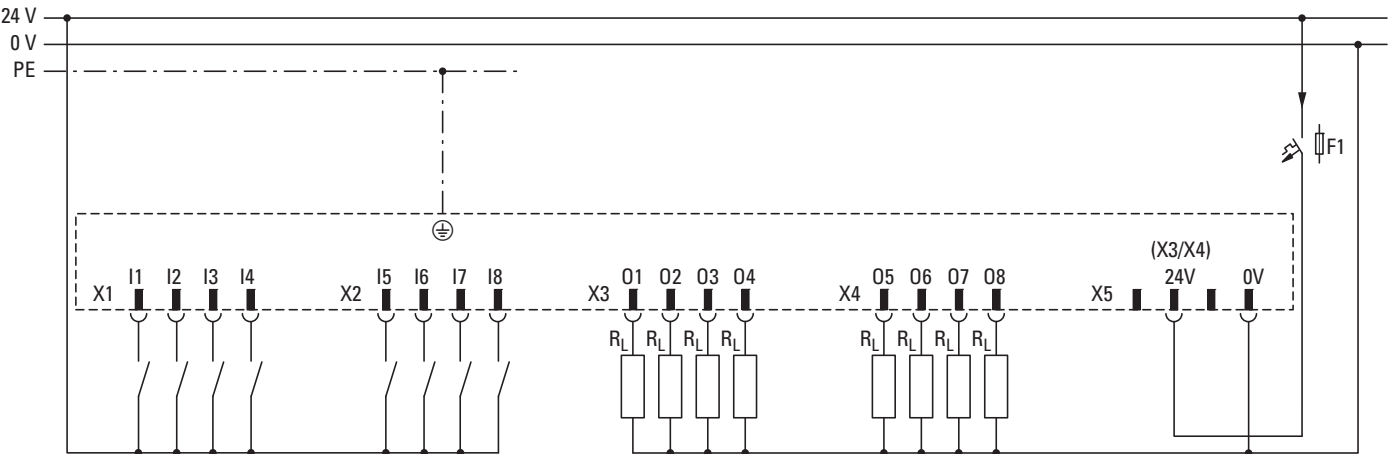
Figure 75: Wiring example showing how to connect inputs to X1/X2 and outputs to X3/X4
