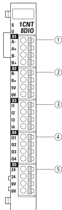
Figure 139: Pin assignment
