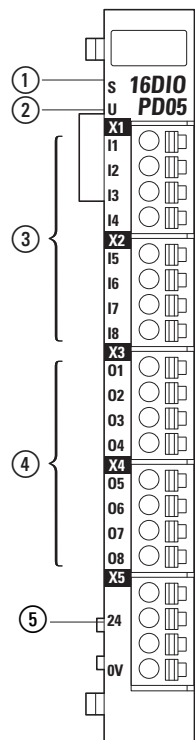
Figure 66: XN-322-16DIO-PD05 LEDs
