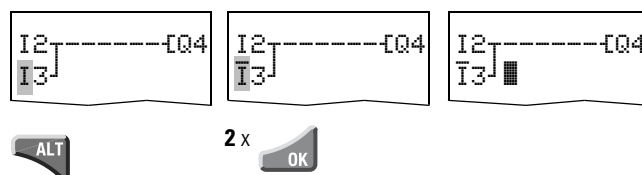
Figure 39: Changing contact I3 from N/O to N/C
