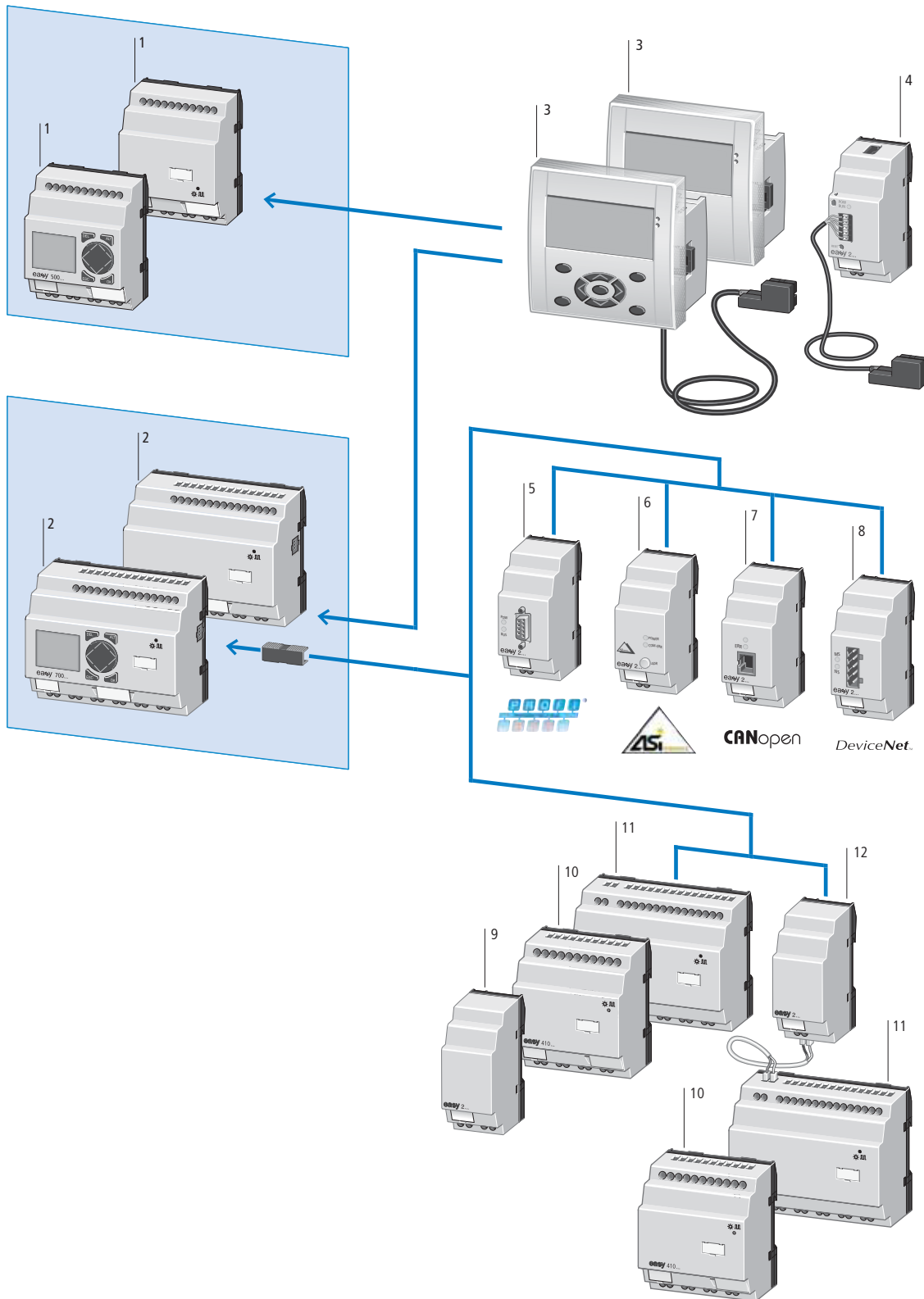
Figure 1: easy basic units and expansion devices
