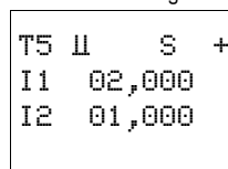
Parameter settings of timing relay T5
