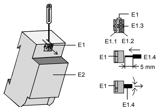
Figure 4: Connecting and disconnecting bus cables
