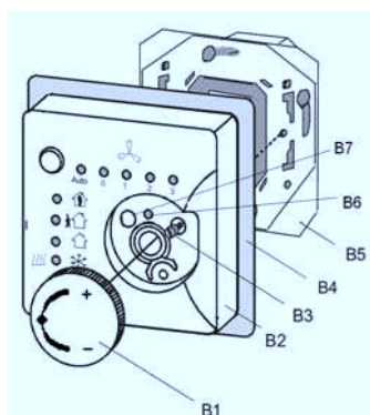
Diagram 3: Mounting the FCU Operator Panel Office
