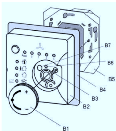
Diagram 1: Mounting the Fan-Coil Unit Operator Panel
