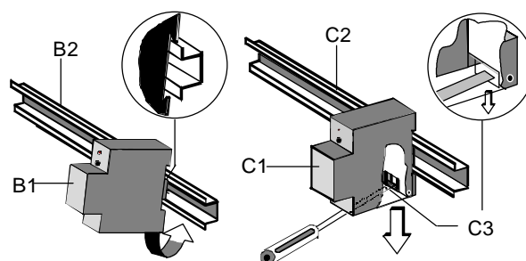
Figure 2: Mounting and dismantling a DIN-rail device
