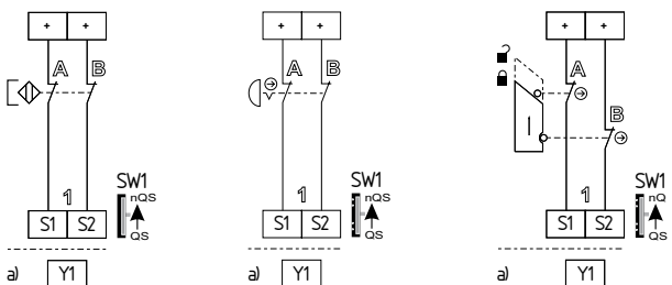
Fig. 11: Magnetic safety switch to IEC 60947-5-3; a) Signalling outputs Fig. 12: Emergency stop circuit to EN ISO 13850 and EN 60947-5-5; a) signal outputs Fig. 13: Guard door monitoring to EN 1088; a) Signalling outputs
