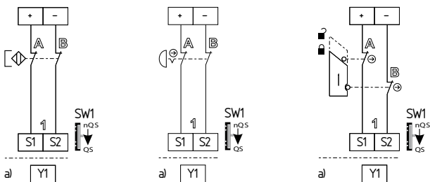
Fig. 8: Magnetic safety switch to IEC 60947-5-3; a) Signalling outputs Fig. 9: Emergency stop circuit to EN ISO 13850 and EN 60947-5-5; a) Signalling outputs Fig. 10: Guard door monitoring to EN 1088; a) Signalling outputs
