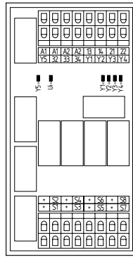
Fig. 3: front view
