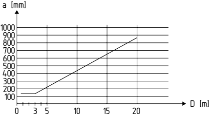
Safety distance a
