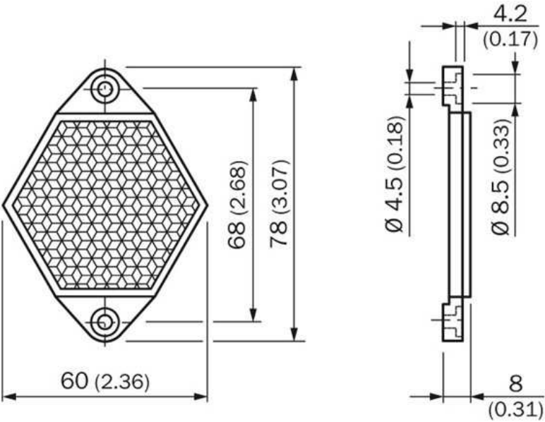
All dimensions in mm (inch)
