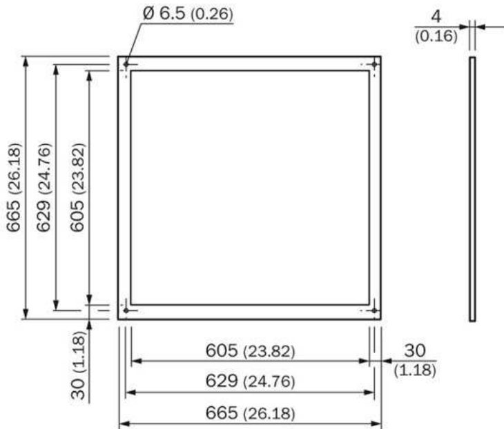
All dimensions in mm (inch)
