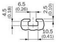
Sliding nut groove for side mounting
