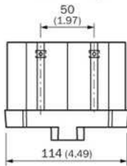
Sliding nut groove for side mounting
