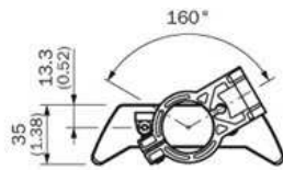
Mounting with swivel mount bracket (Part no. 2019659)
