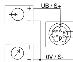
5-pin plug
