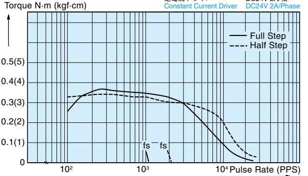
TS3653N2E4,N12E4
