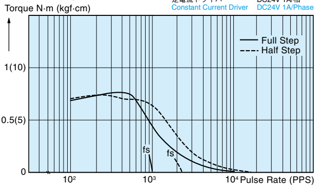
TS3653N2E6,N12E6
