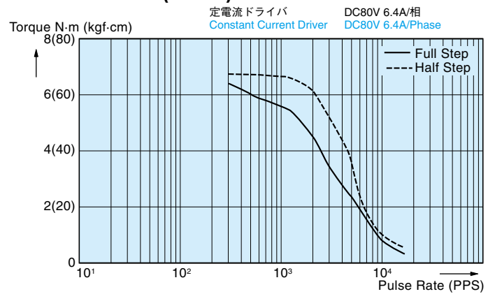
TS3684N2E6 (TYPE2)
