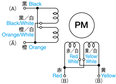
TYPE 2 バイポーラ(パラレル結線) BIPOLAR (Parallel connection)
