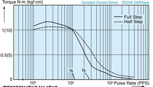
TS3653N4E12,N14E12
