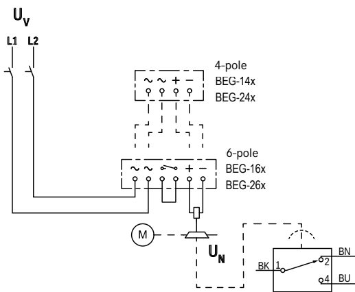
Supply: Phase-Phase
