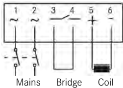
AC switching
