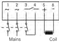
DC switching
