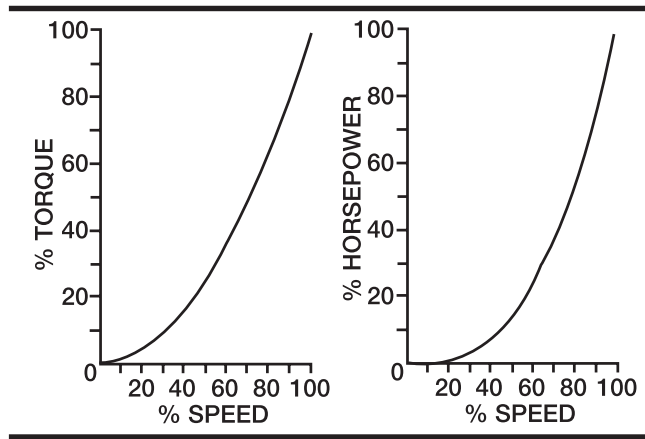
Variable Torque — Speed-Torque Relationships Figure 7
